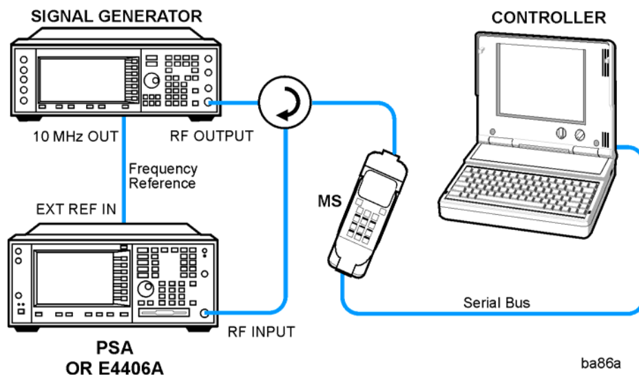
Figure 2-44 Spectrum Measurement System
