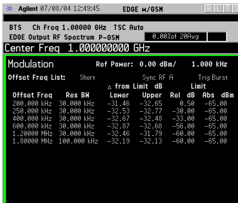
Figure 2-10 EDGE ORFS Result - Example (Short List) Modulation Margin & Limits View
