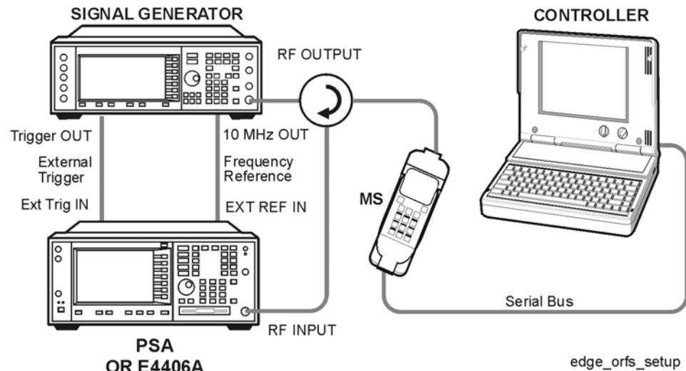
Figure 2-20 GSMK ORFS Measurement System
