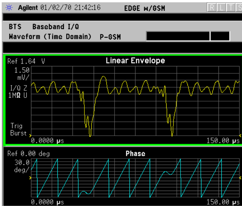
Figure 2-61 Waveform Measurement - I and Q Waveform View
