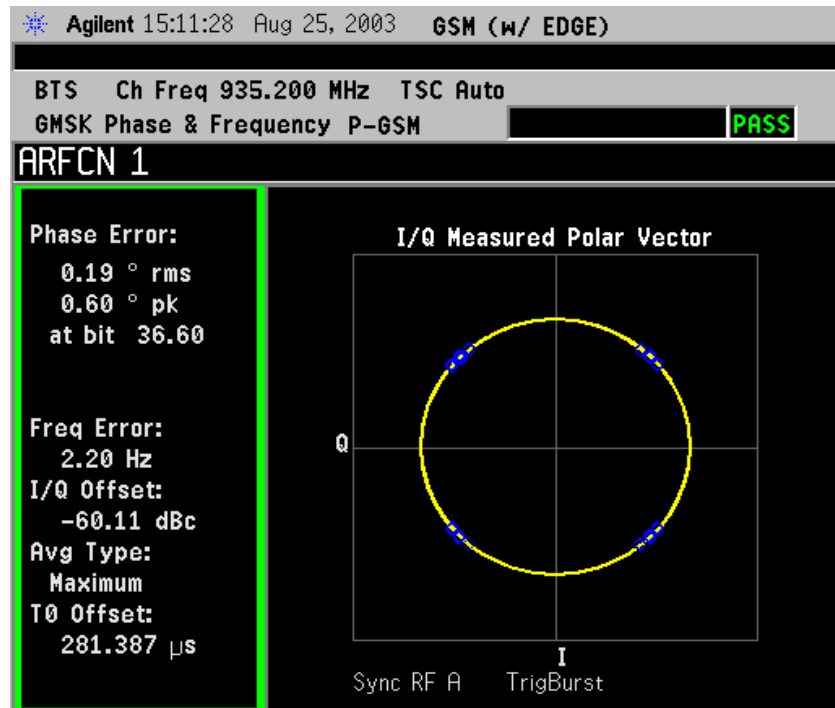
Figure 3-20 GSM Phase and Frequency Error Result - Polar Vector View
