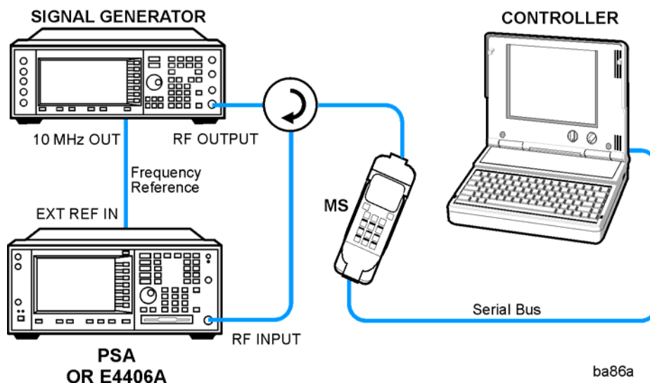
Figure 2-36 GMSK Pwr vs Time T Measurement System
