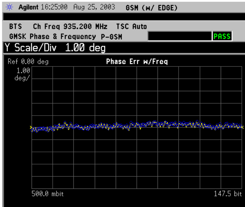
Figure 2-32 GMSK Phase and Frequency Error Result - Phase Error View
