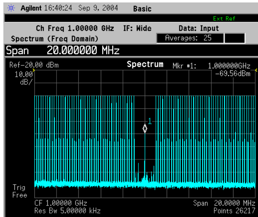
Figure 2-52 Spectrum Measurement - Spectrum View with Opt. 122– 80 MHz Bandwidth Digitizer Hardware
