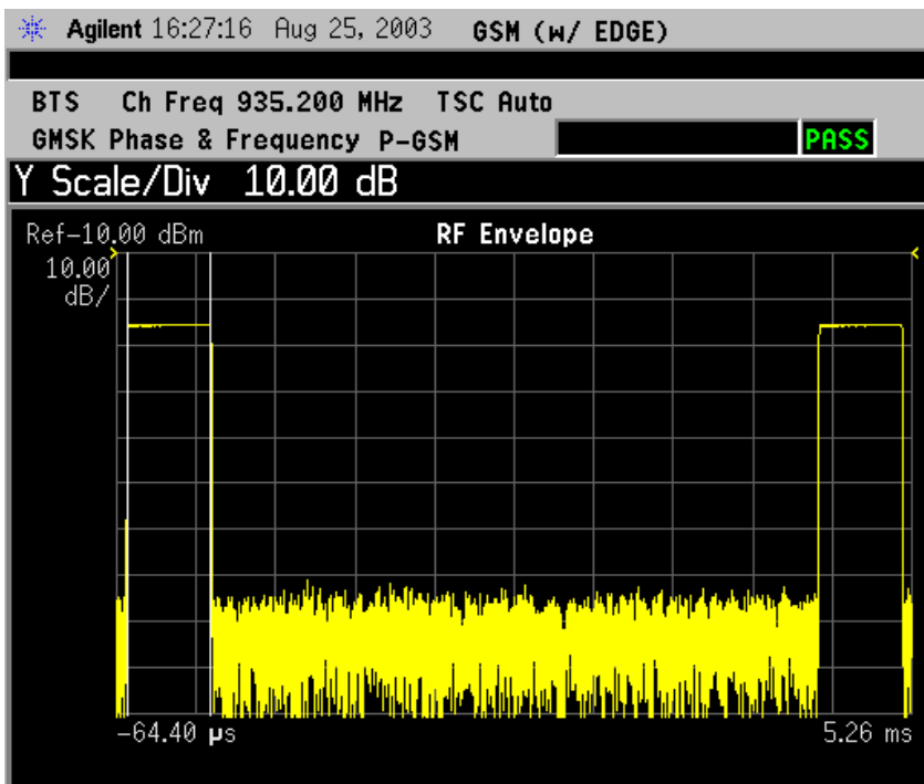
Figure 2-33 GMSK Phase and Frequency Error Result - RF Envelope View
