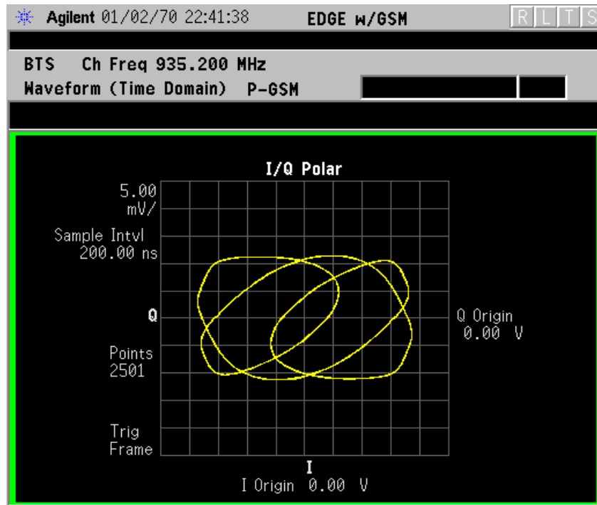
Figure 2-62 Waveform Measurement - I/Q Polar View
