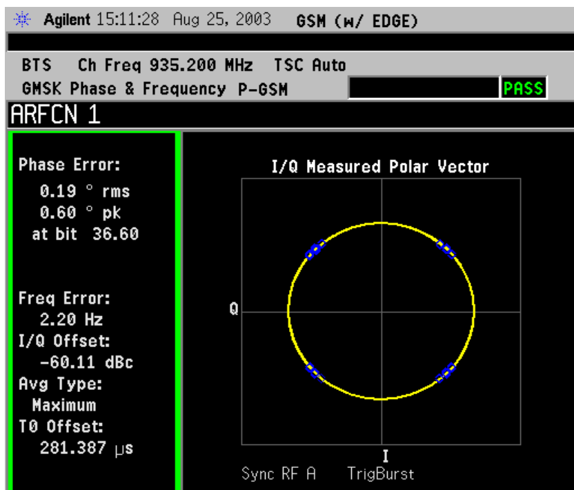
Figure 2-34 GMSK Phase and Frequency Error Result - Polar View
