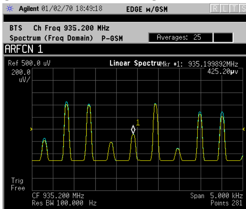
Figure 2-47 Spectrum Measurement - Linear Spectrum View (for E4406A)
