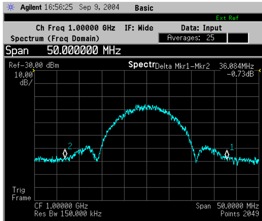
Figure 2-51 Spectrum Measurement - Spectrum Zoom View with Opt. 122–80 MHz Bandwidth Digitizer Hardware
