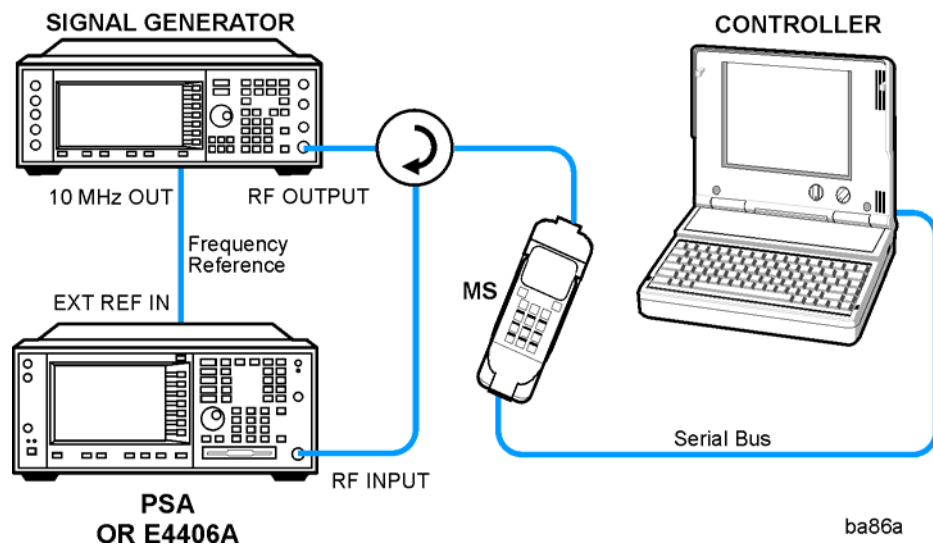
Figure 2-57 Waveform Measurement System
