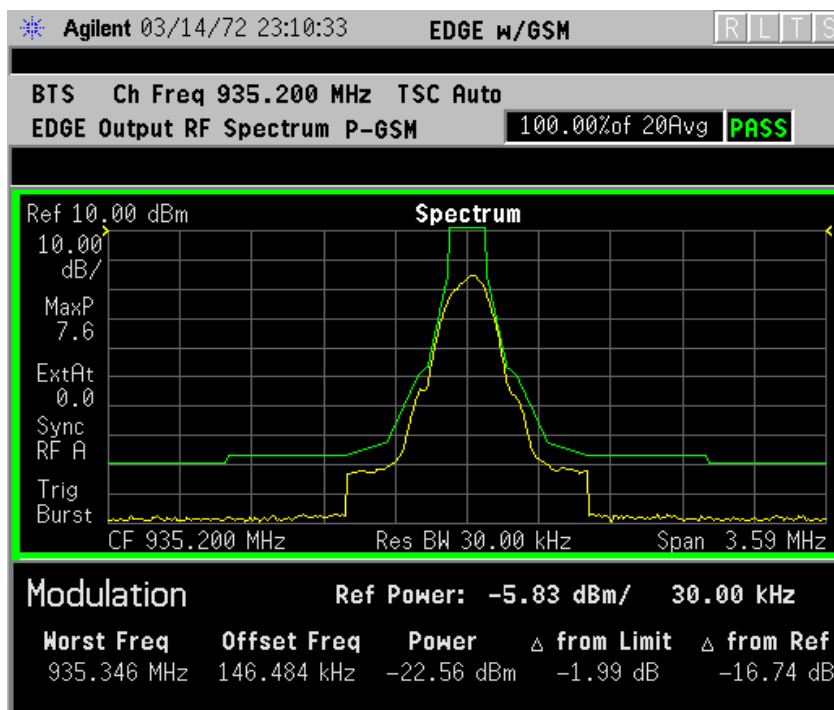
Figure 2-16 EDGE ORFS Result - Example Modulation Swept View
