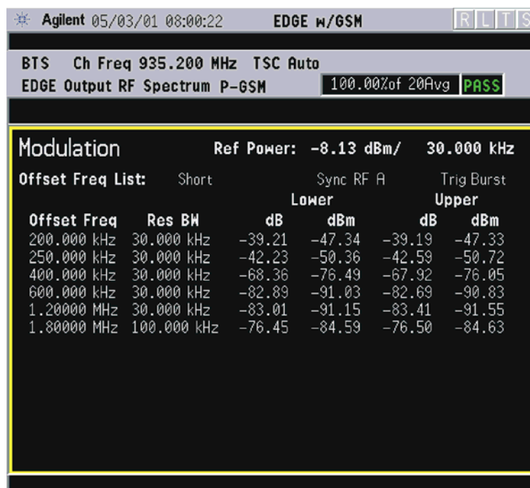
Figure 2-9 EDGE ORFS - Example (Short List) Modulation Power View
