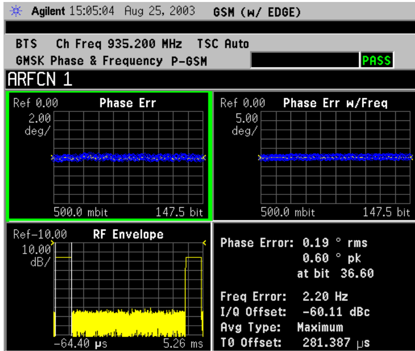
Figure 2-31 GMSK Phase and Frequency Error Result - Quad View
