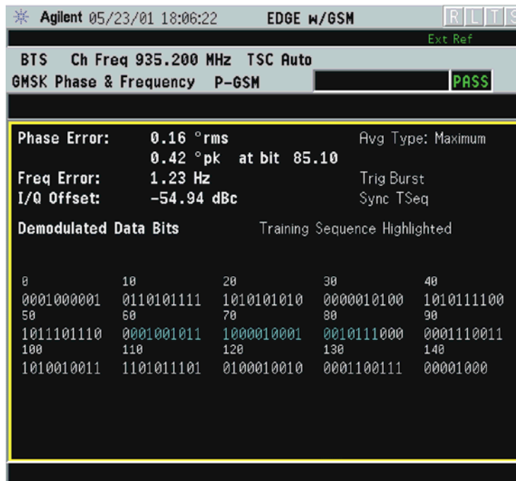
Figure 2-35 GSMK Phase and Frequency Error Result - Data Bits
