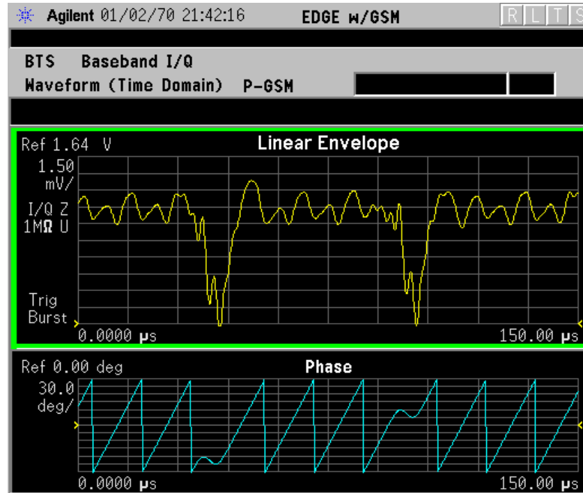
Figure 3-33 Waveform Measurement - Linear Envelope View
