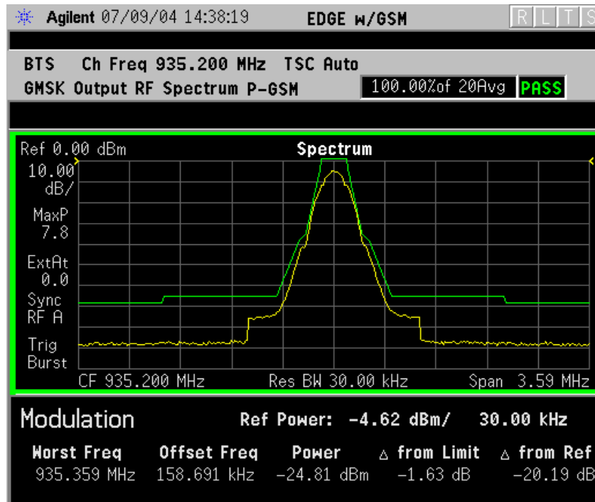
Figure 2-28 GMSK ORFS Result - Example Modulation Swept View
