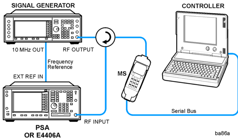
Figure 2-42 GMSK Transmitter Band Spurious Measurement System
