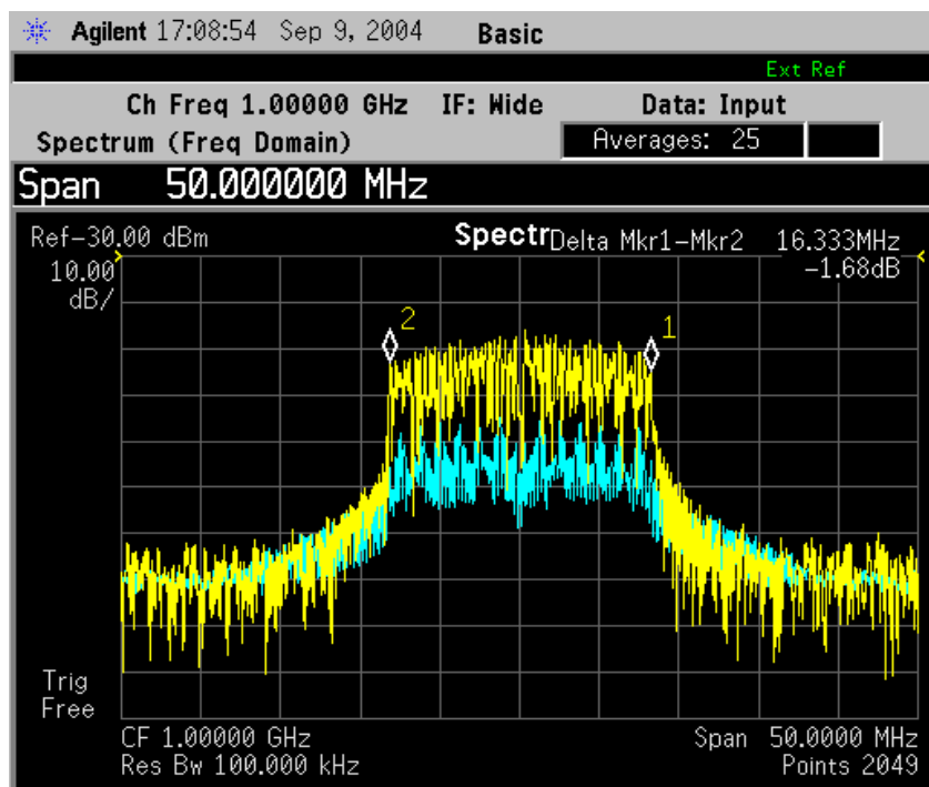
Figure 2-50 Spectrum Measurement - Spectrum Zoom View with Opt. 122–80 MHz Bandwidth Digitizer Hardware
