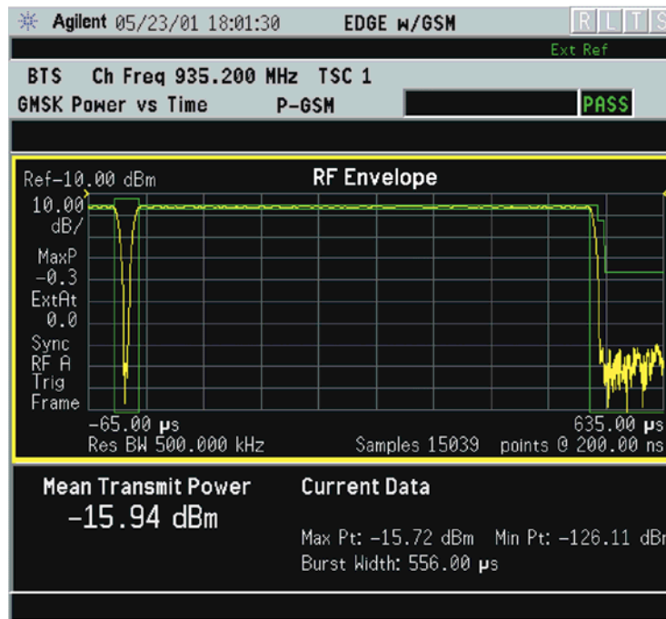
Figure 2-37 GMSK Power vs. Time Result - Burst View
