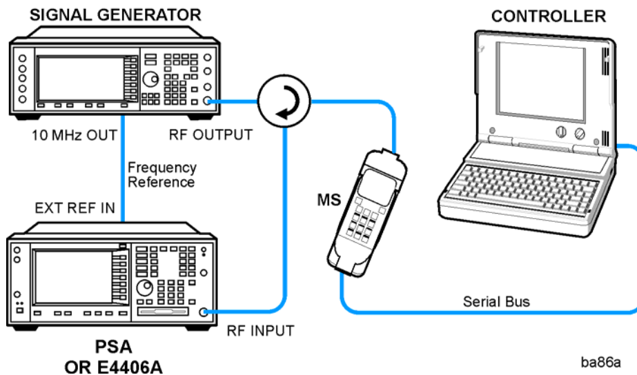
Figure 2-6 EDGE EVM Measurement System
