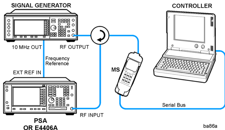
Figure 2-30 GMSK Phase and Frequency Measurement System
