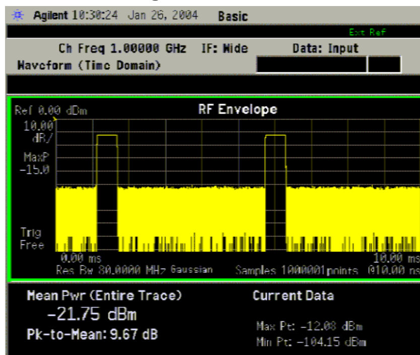
Figure 2-63 Waveform Measurement - RF Envelope View with Opt. 122– 80 MHz Bandwidth Digitizer Hardware
