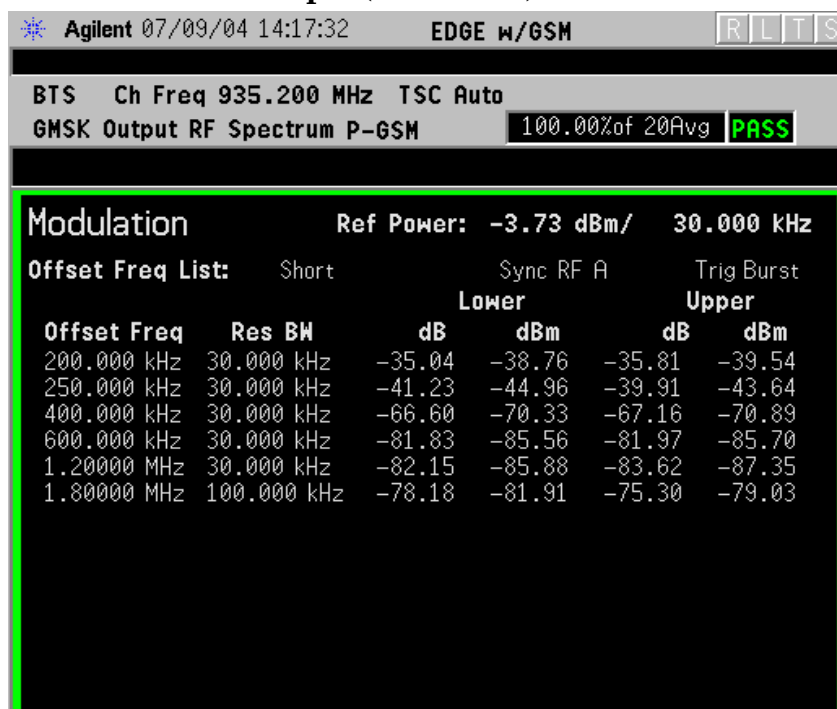
Figure 2-21 GMSK ORFS - Example (Short List) Modulation Power View
