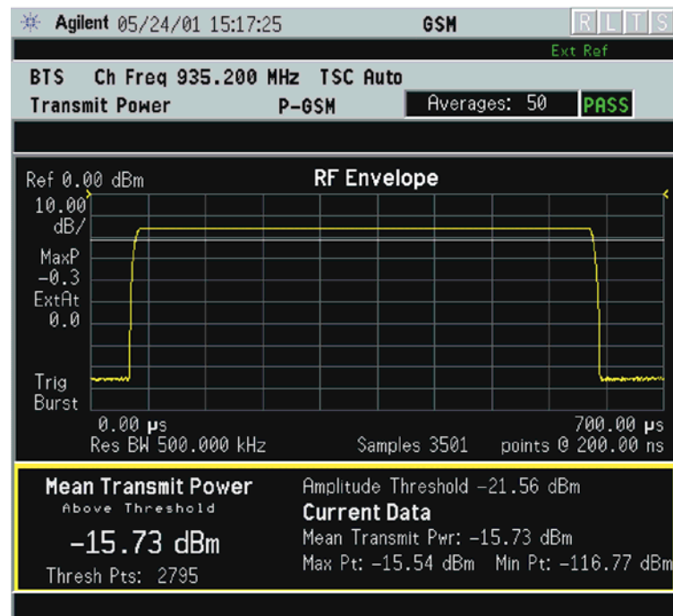
Figure 3-31 Transmit Power Result - Single Burst (with data table)
