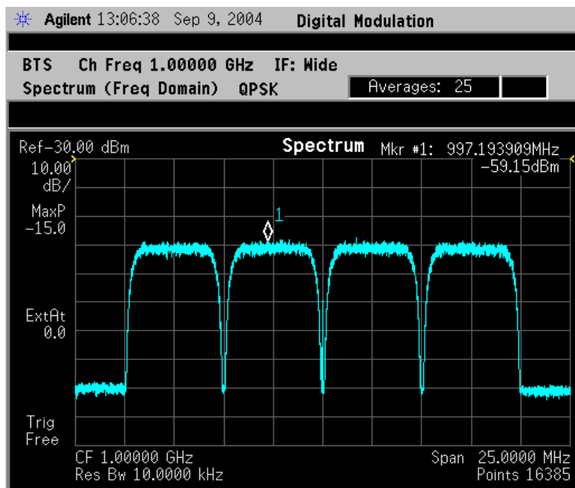
Figure 2-53 Spectrum Measurement - Spectrum Zoom View with Opt. 122–80 MHz Bandwidth Digitizer Hardware
