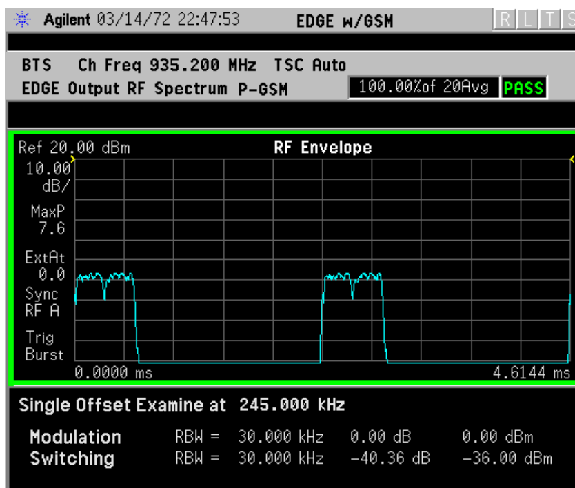
Figure 2-14 EDGE ORFS Result - Switching Single Offset (Examine) View
