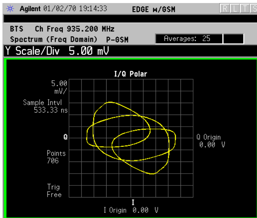
Figure 2-49 Spectrum Measurement - I/Q Polar View (for E4406A)
