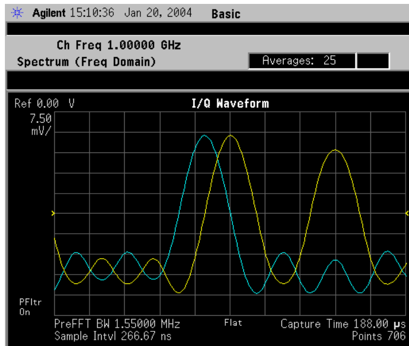
Figure 3-27 Spectrum Measurement - I/Q Waveform (Time Domain) Result (E4406A View)
