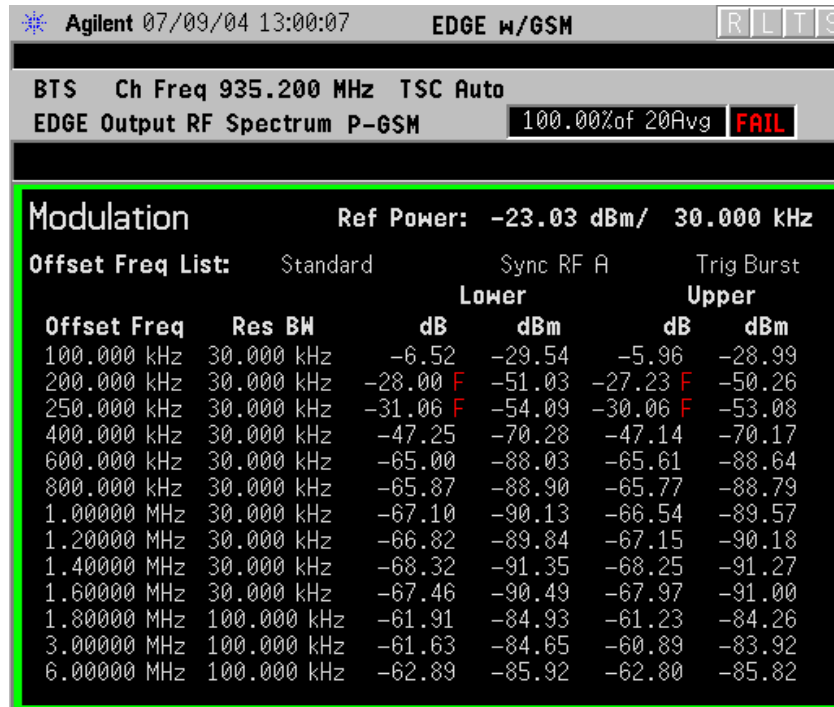
Figure 2-17 EDGE ORFS Result - Full Frame Modulation (FAST) View
