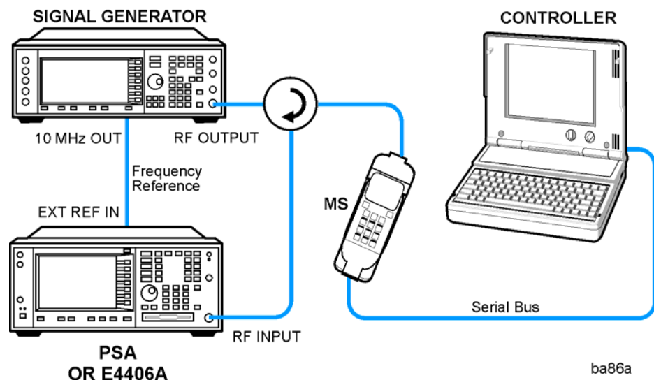
Figure 2-54 Transmit Power Measurement System
