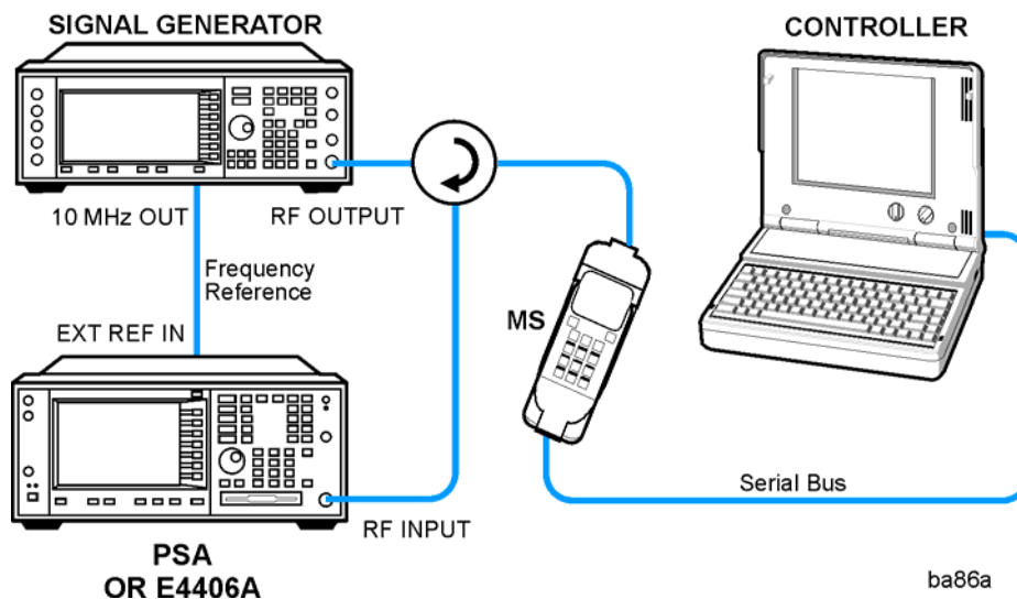
Figure 2-18 EDGE Transmitter Band Spurious Measurement System
