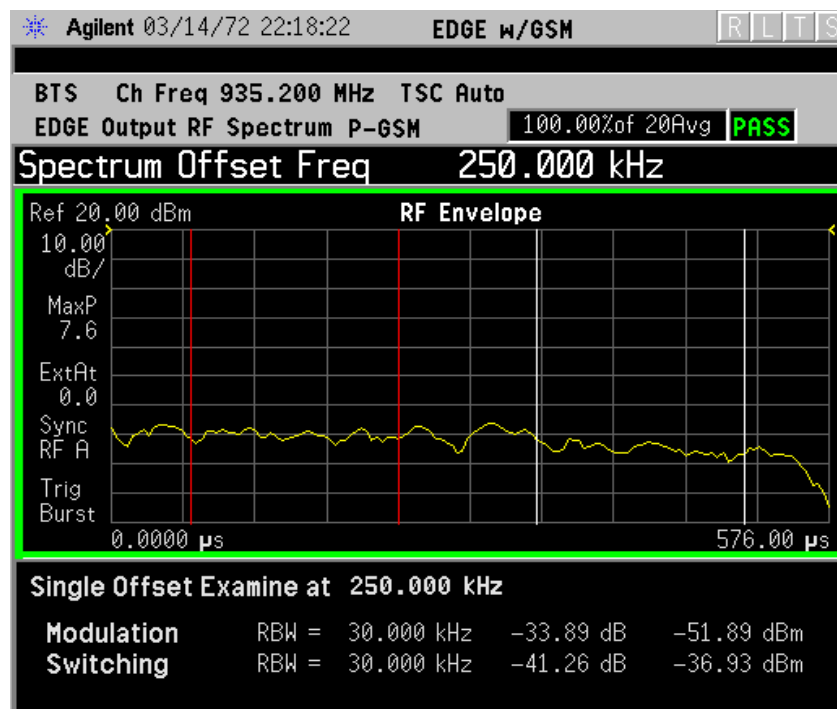
Figure 2-13 EDGE ORFS Result - Modulation Single Offset (Examine) View
