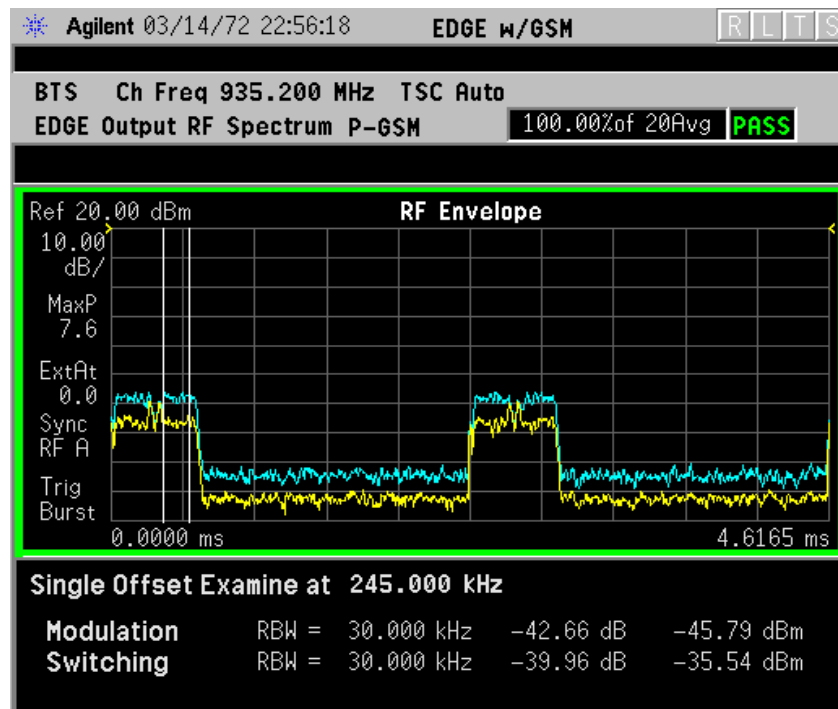
Figure 2-15 EDGE ORFS Result - Mod & Switch Single Offset (Examine) View
